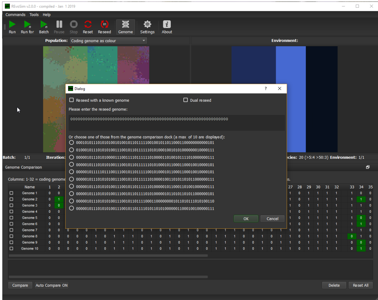
Fig. 7: Reseed dialog showing first ten genomes as selected in the Genome Comparison Dock (created with v2.0.0).
