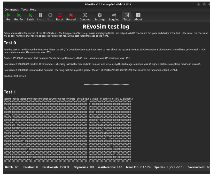
Fig. 11: REvoSim main window in test mode.
